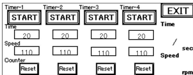
Touch panel view for Multi timer polishing mode
