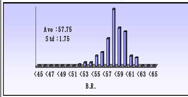
Distribution of B.R. for HF07 Laping fim(1550nm)
